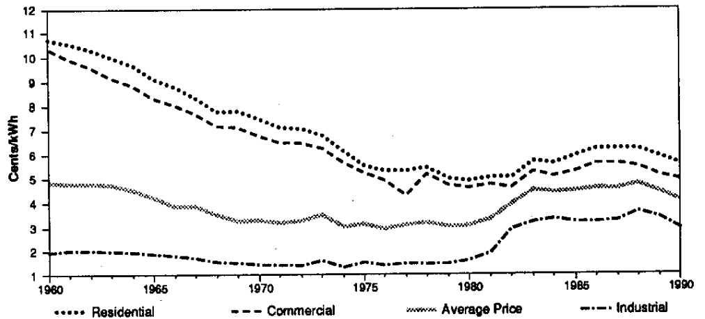
Figure 2.6. Real Electricity Prices, 1960-90 (1991 dollars)
