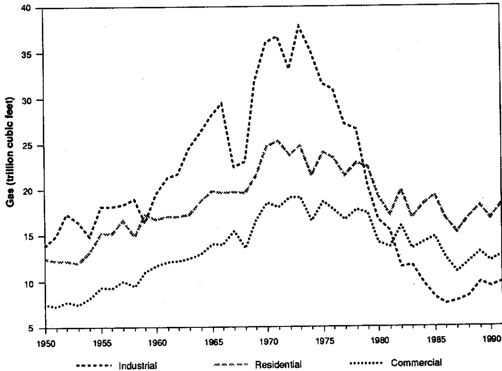
Figure 4.4. Natural Gas Consumption by Customer Class, 1950-91
