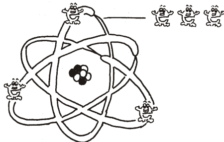
Figure 1. Electricity is the flow of charged particles
