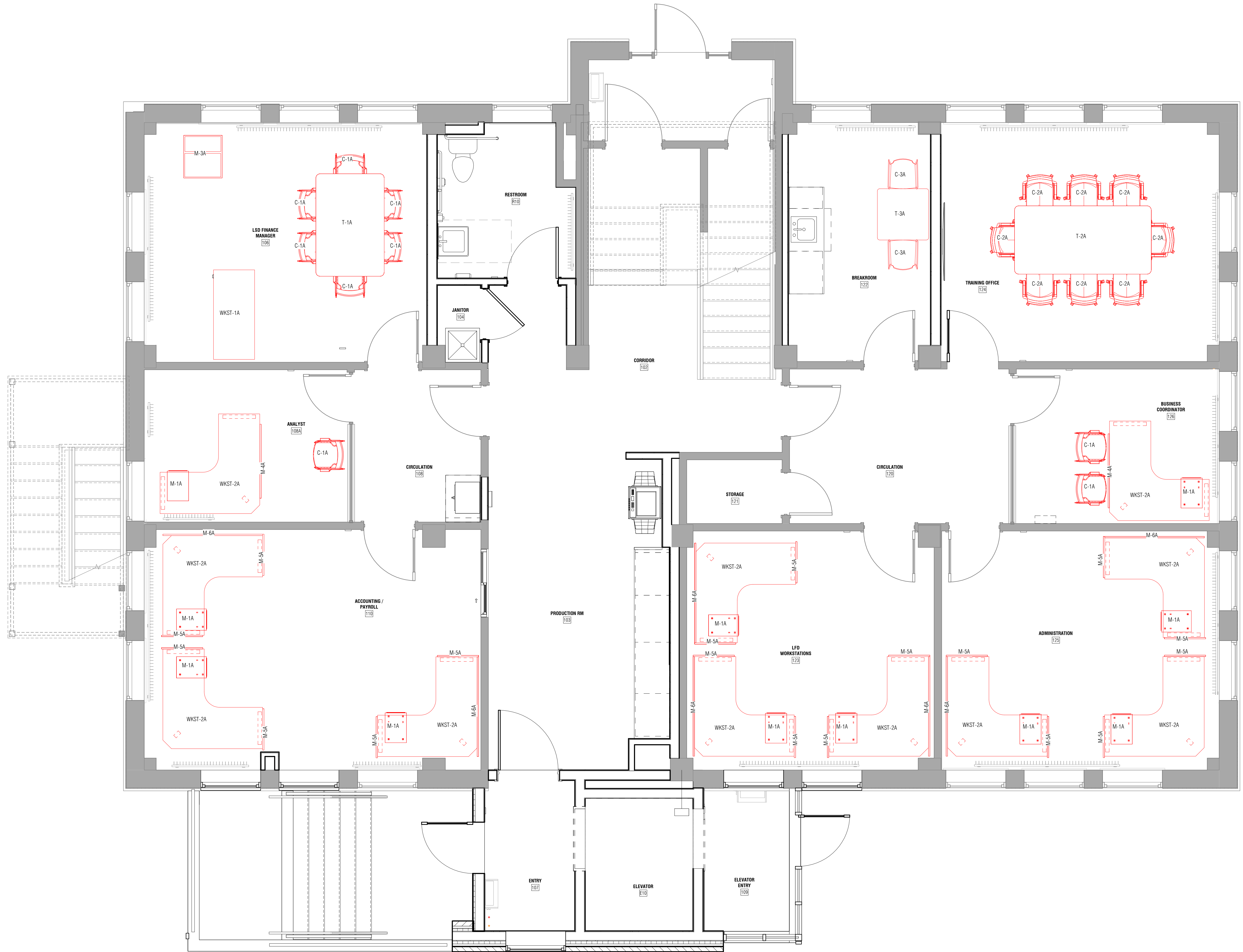
12.00 FURNITURE PLAN - FIRST FLOOR 3/8" = 1'-0"
