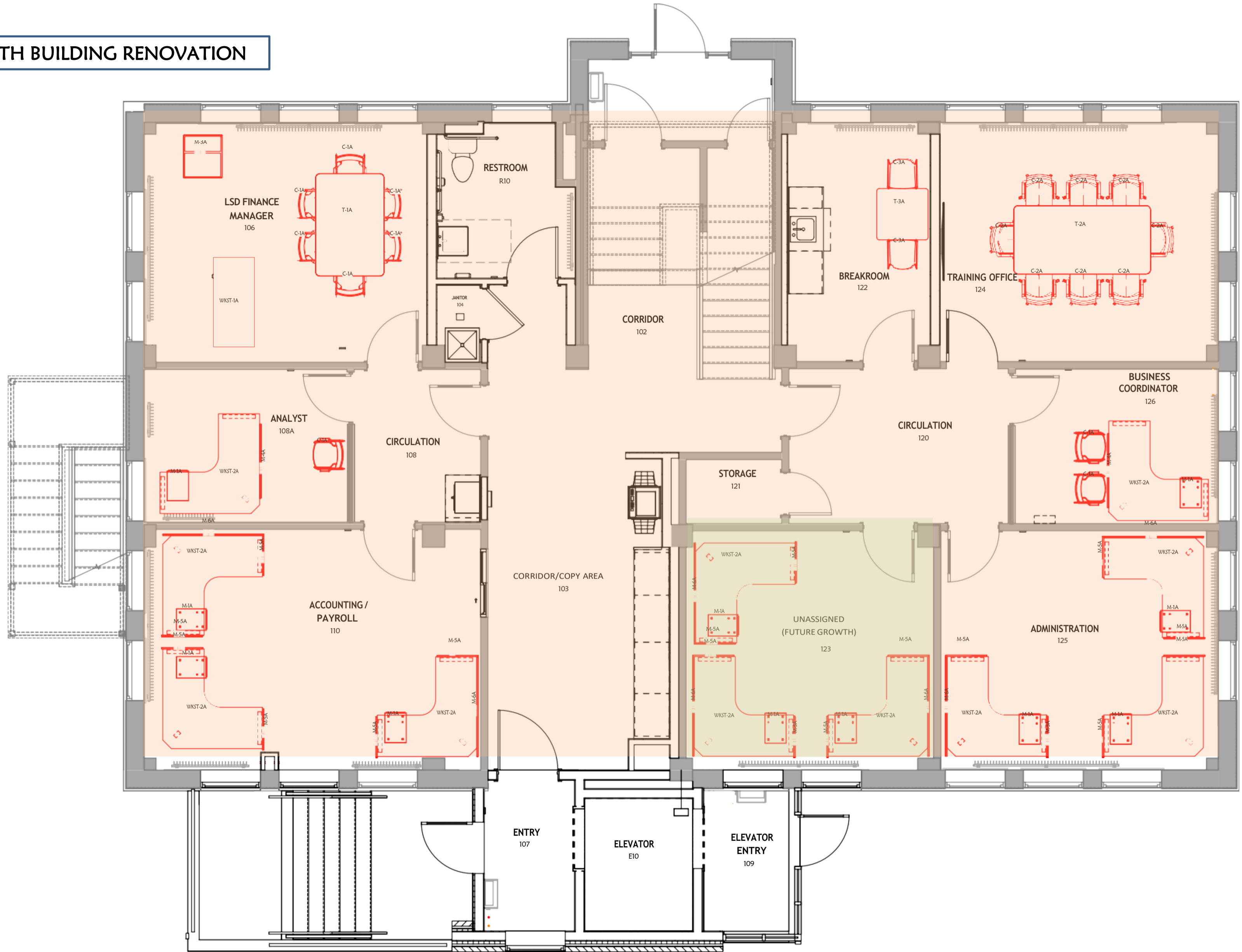
FURNITURE PLAN - FIRST FLOOR
