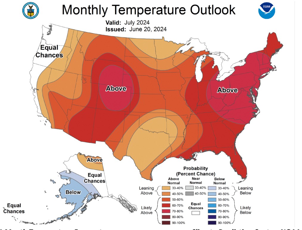
Figure 10 - 1 Month Temperature Forecast:
