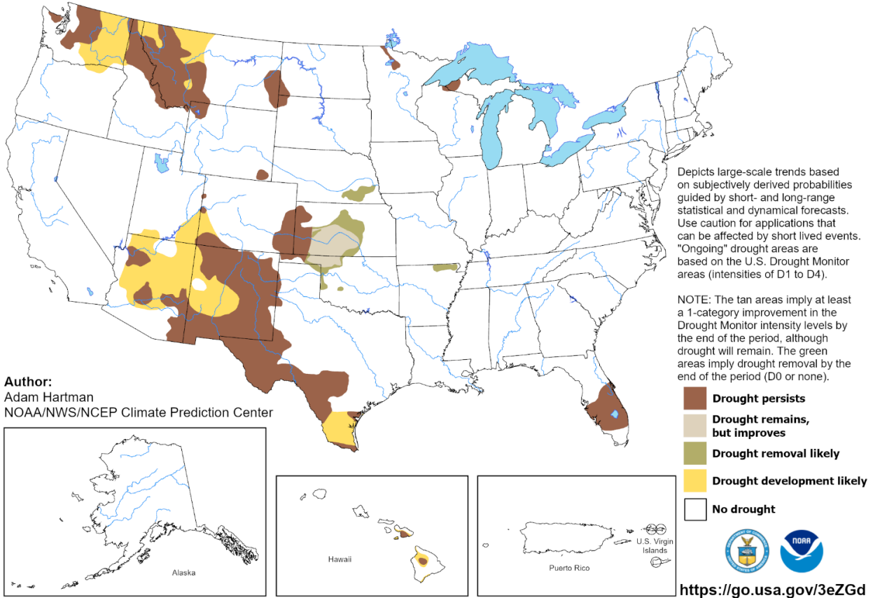
Figure 5 – U.S. Monthly Drought Outlook
