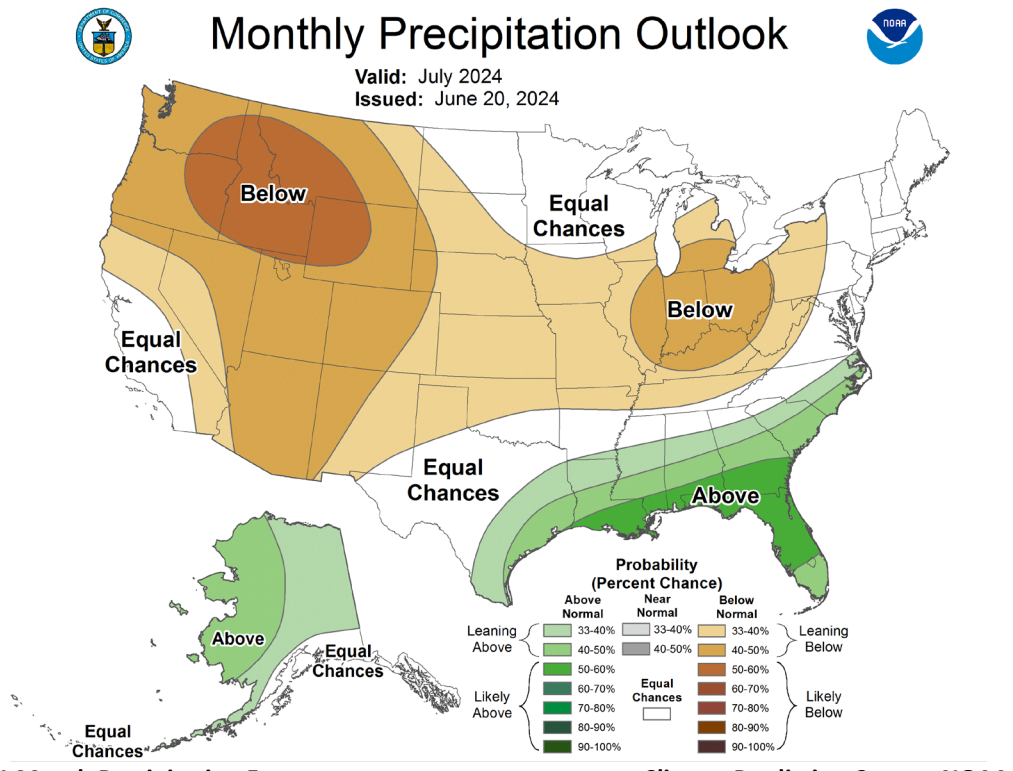
Figure 11 - 1 Month Precipitation Forecast:
